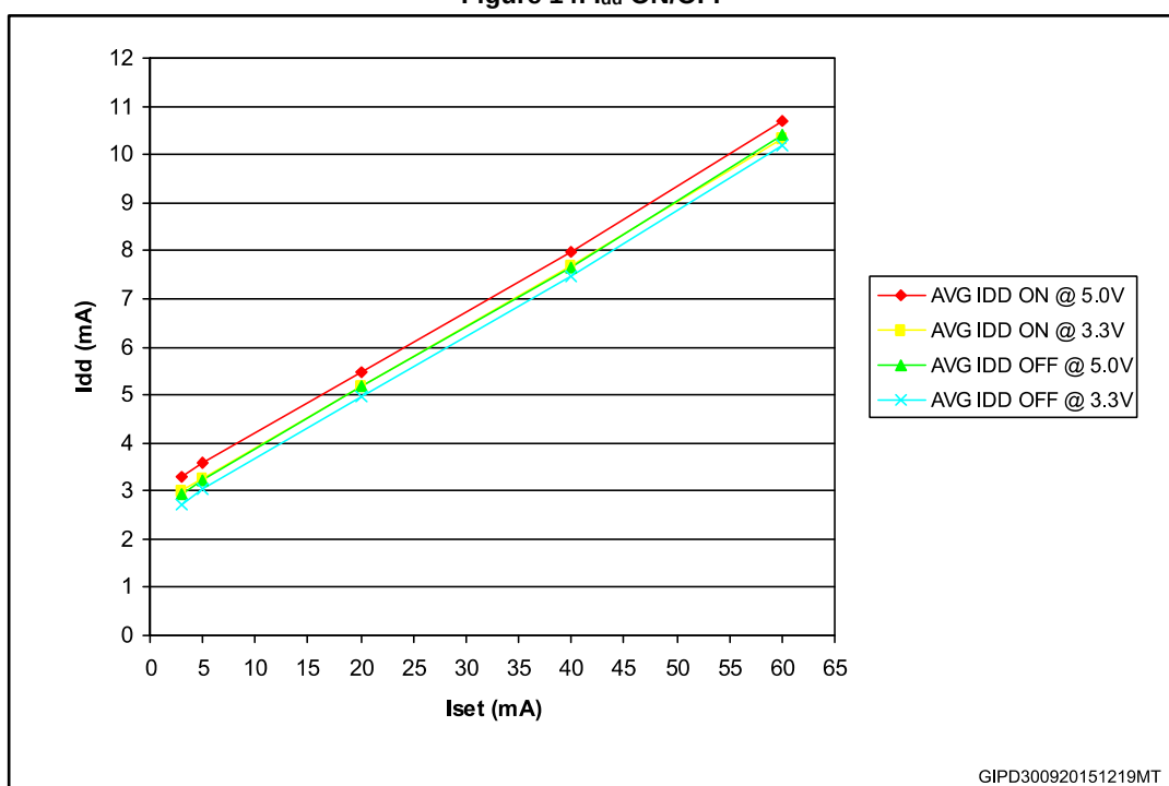
Figure 14: I_{dd} ON/OFF
