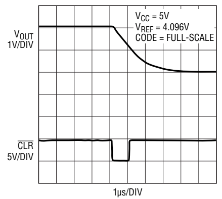
Hardware \overline{CLR} to Mid-Scale
