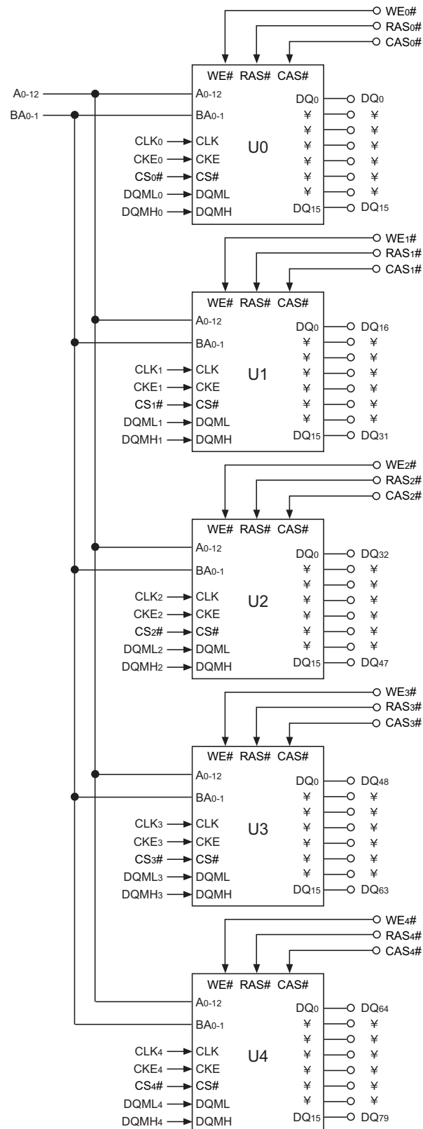
FIGURE 2 – FUNCTIONAL BLOCK DIAGRAM
