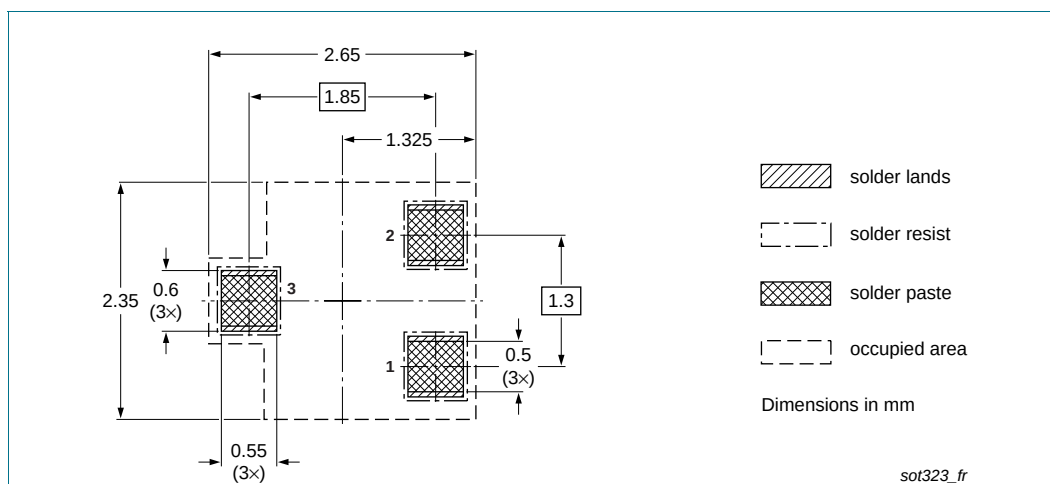
Fig 8. Reflow soldering footprint SOT323 (SC-70)
