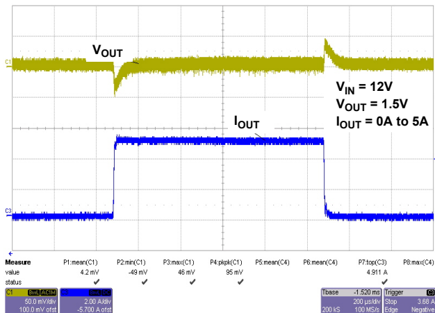
FIGURE 9. 1.5V TRANSIENT RESPONSE
