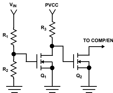
FIGURE 24. SEQUENCE CIRCUIT
