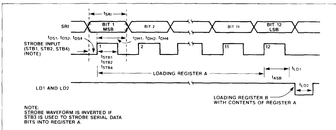
Figure 6. Timing Diagram
