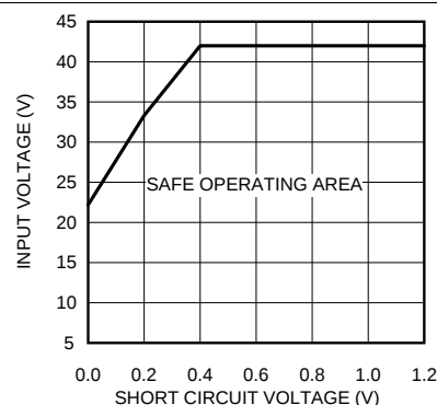
Figure 16. SOA 500 kHz
