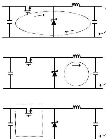
Figure 22. Current Flow in a Buck Application
