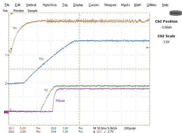
Fig.15: Start-up sequence into 60A load. Ch 1 : V_{in} , Ch 2 : V_{ss} , Ch 3 : Power Good, Ch 4 : V_o
