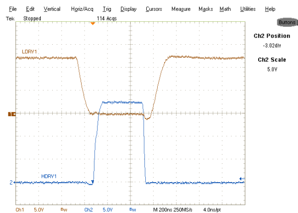
Fig. 27: HDRV1 and LDRV1 at 20A. Ch 1 : LDRV1, Ch 2 : HDRV1
