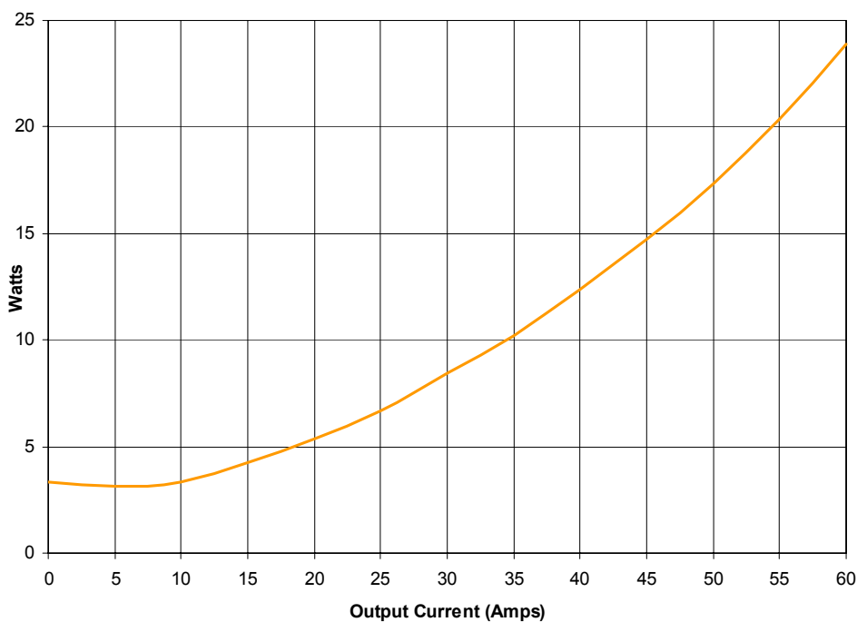
Fig. 34: Power loss versus load current at 45^\circ\text{C} with heat sink and 200LFM air flow
