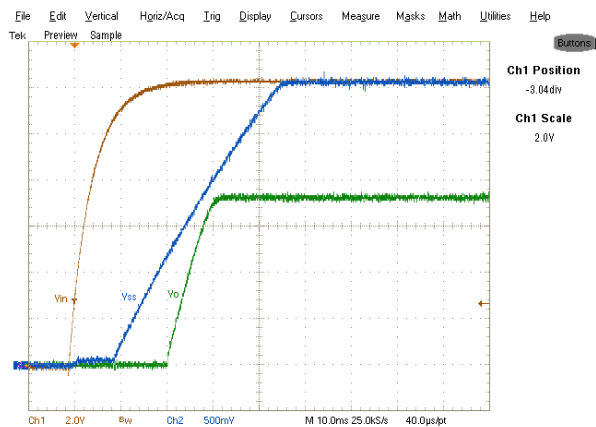
Fig.13: Start-up sequence at no load. Ch 1 : V_{in} , Ch 2 : V_{ss} , Ch 4 : V_o
