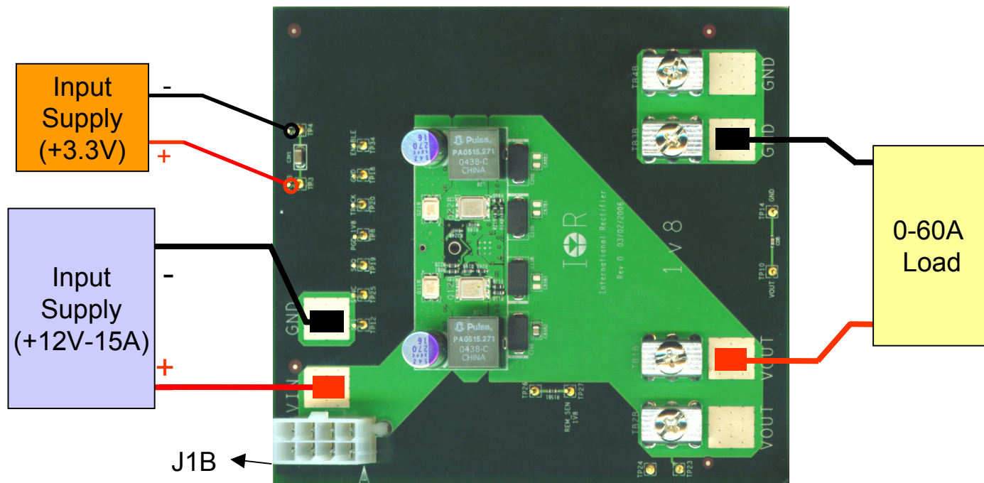
Fig. 1: Connection diagram of the IRDC3622S evaluation board.
