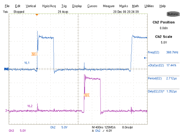
Fig. 32: Inductor points at 60A load.
