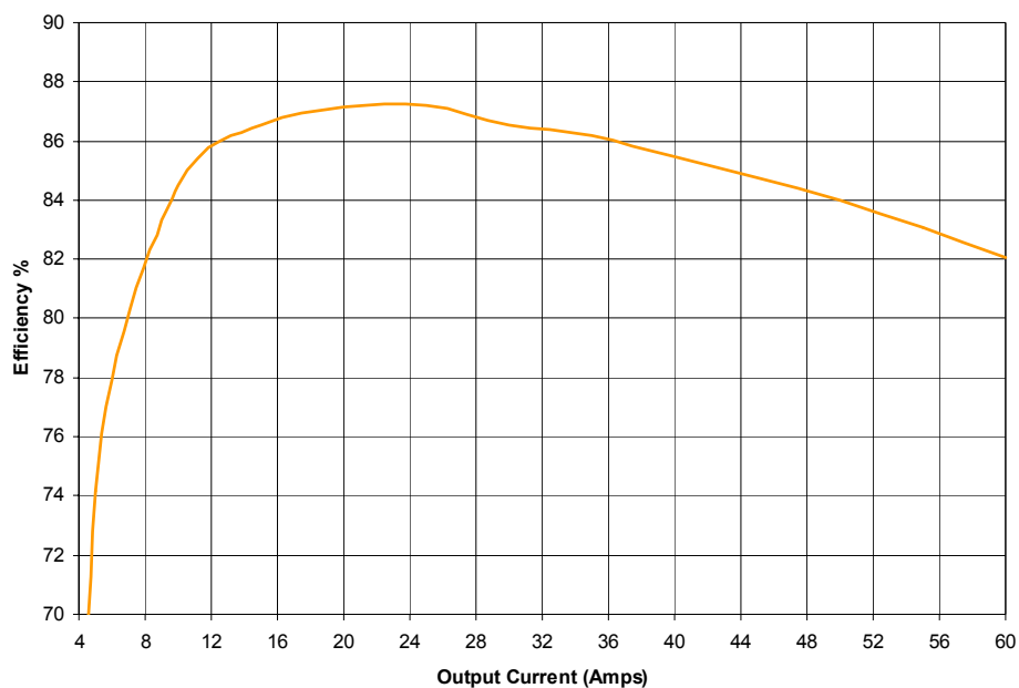
Fig. 33: Efficiency versus load current at 45^\circ\text{C} with heat sink and 200LFM air flow.
