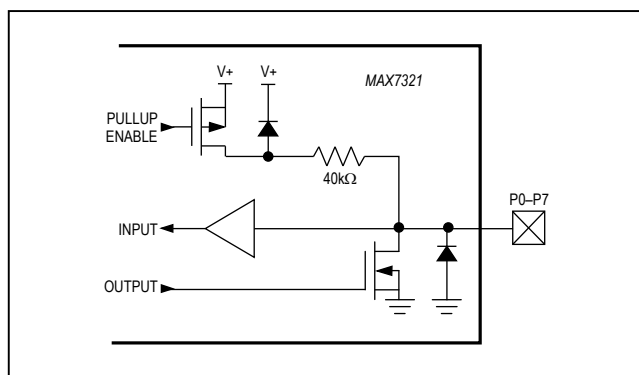
Figure 9. MAX7321 I/O Structure
