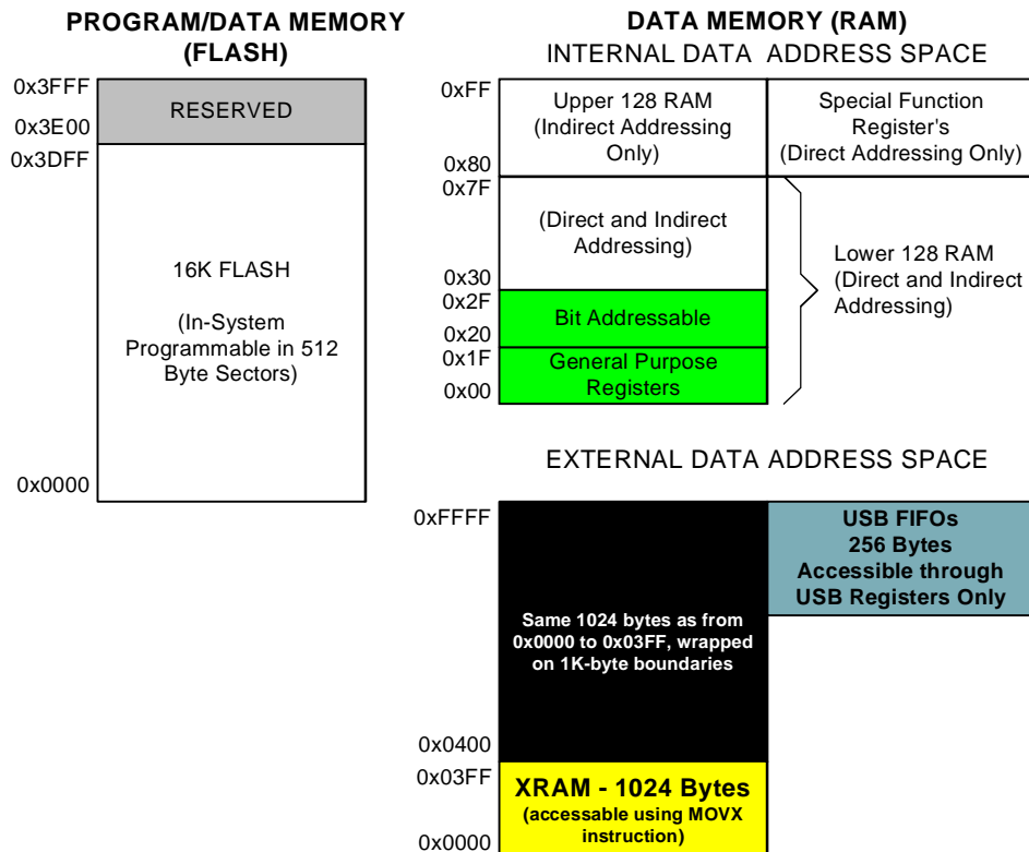
Figure 6.2. Memory Map
