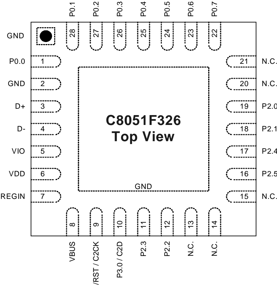
Figure 4.1. C8051F326 QFN-28 Pinout Diagram (Top View)
