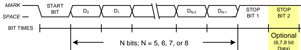
Figure 13.2. UART0 Timing Without Parity or Extra Bit
