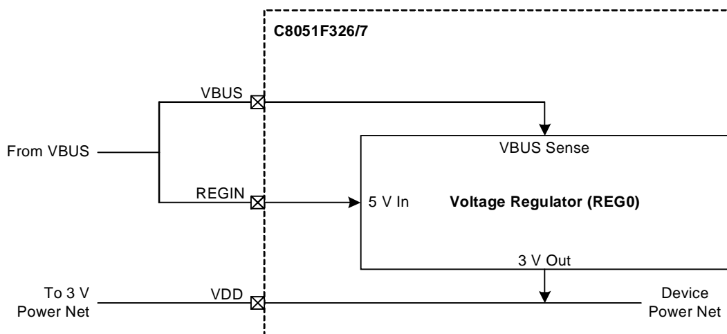
Figure 5.1. REG0 Configuration: USB Bus-Powered
