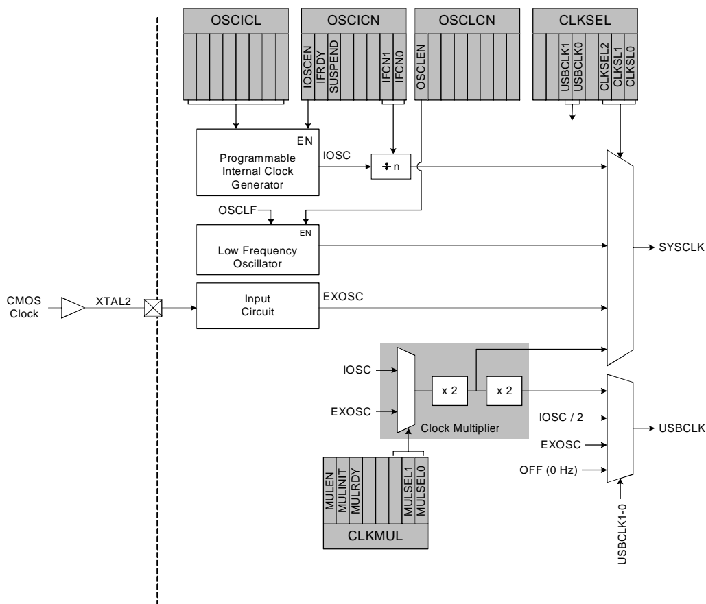
Figure 10.1. Oscillator Diagram
