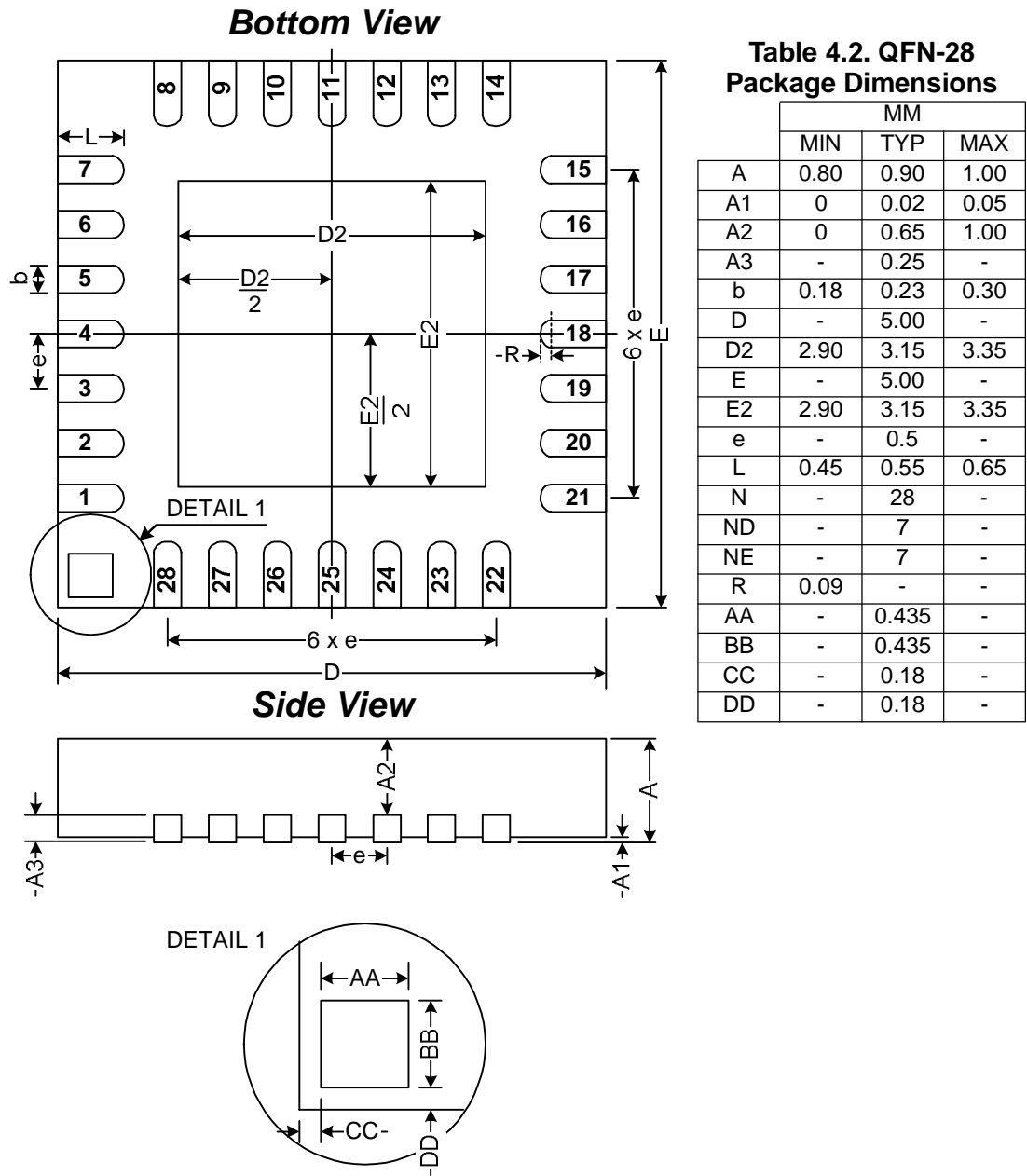
Figure 4.3. QFN-28 Package Drawing
