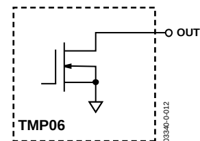
Figure 30. TMP06 Digital Output Structure
