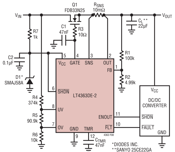
Figure 8. Overvoltage Regulator with Input Voltage Detection
