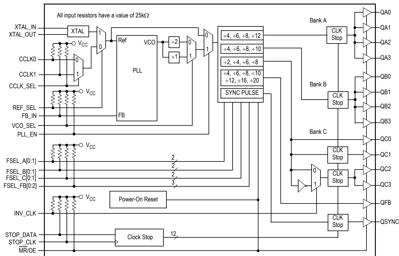
Figure 1. Logic Diagram
