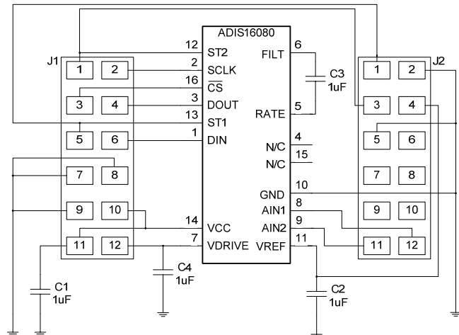
Figure 1 - ADIS16080/PCB Schematic
