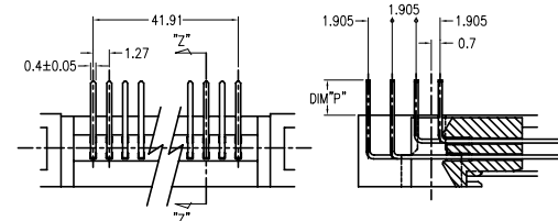
VIEW "Y"-Y"(4/1)
