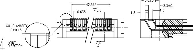
VIEW "Y"- "Y"(4/1)
