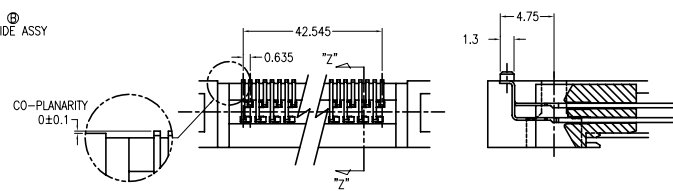
VIEW "Y"- "Y"(4/1)
