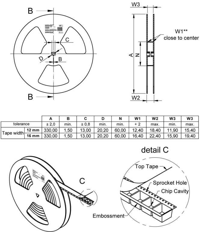
sectional drawing B-B
