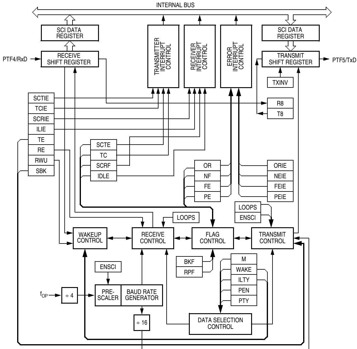
Figure 13-2. SCI Module Block Diagram
