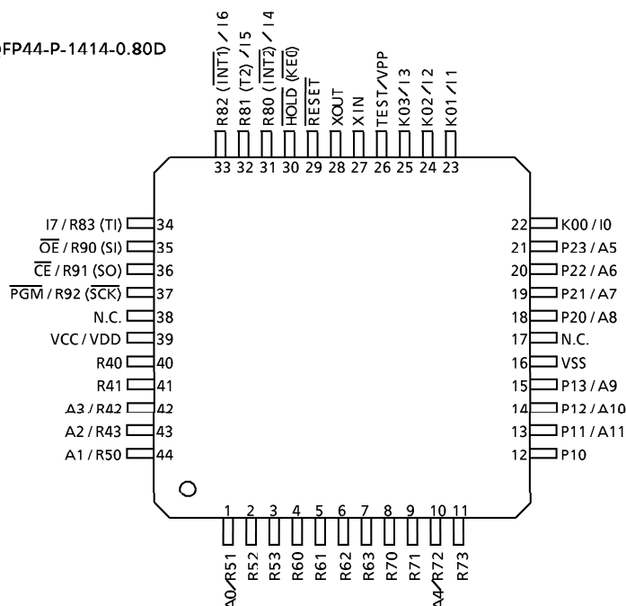
QFP44-P-1414-0.80D
