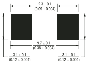
Recommended Pad Layout MF-SM030, 050, 075, 075/60, 100, 100/33, 125, 260, 300
