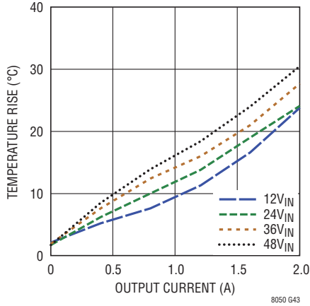
Internal Temperature Rise vs Output Current, 8V OUT
