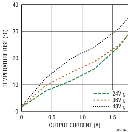
Internal Temperature Rise vs Output Current, 18V OUT
