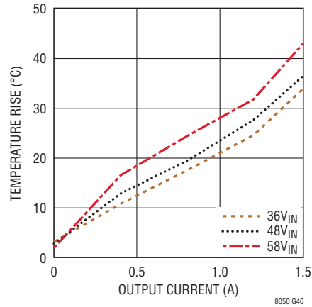
Internal Temperature Rise vs Output Current, 24V OUT
