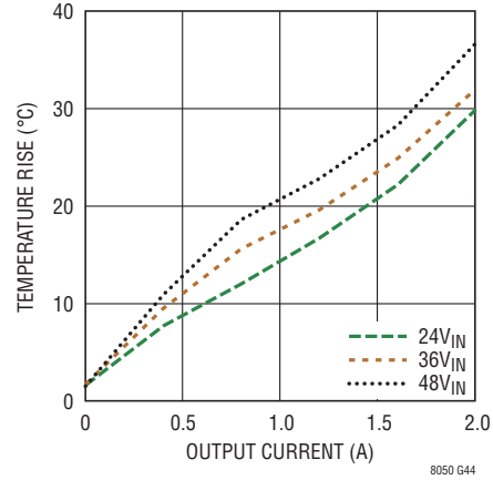
Internal Temperature Rise vs Output Current, 12V OUT
