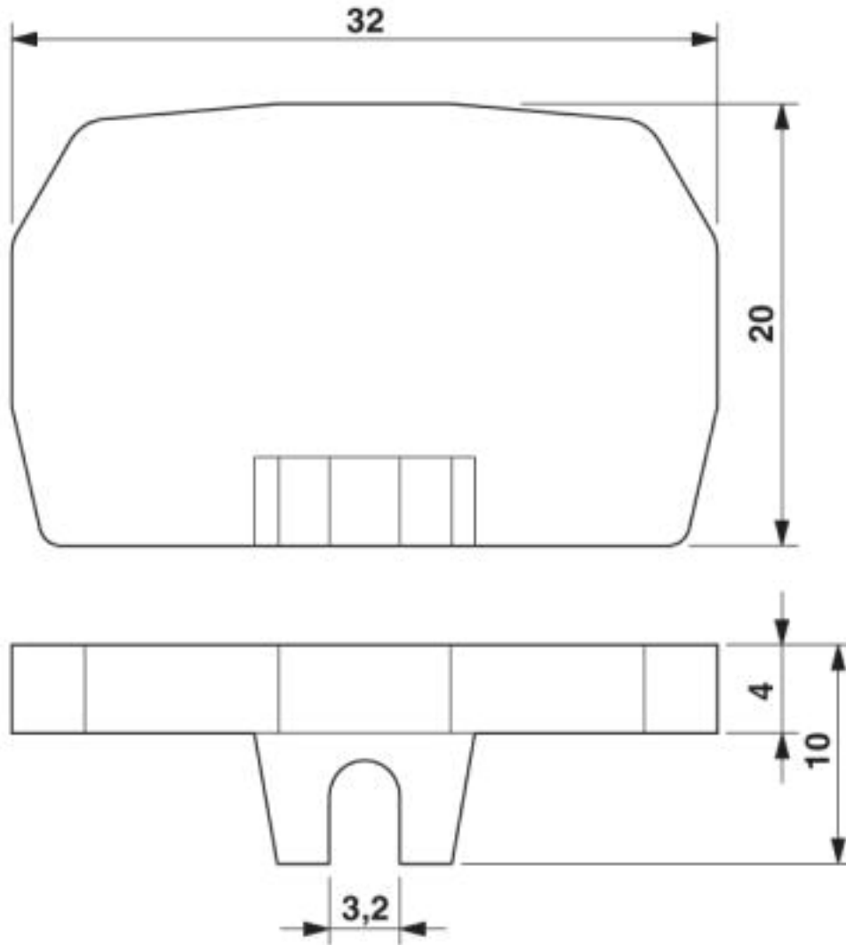
Dimensional drawing
