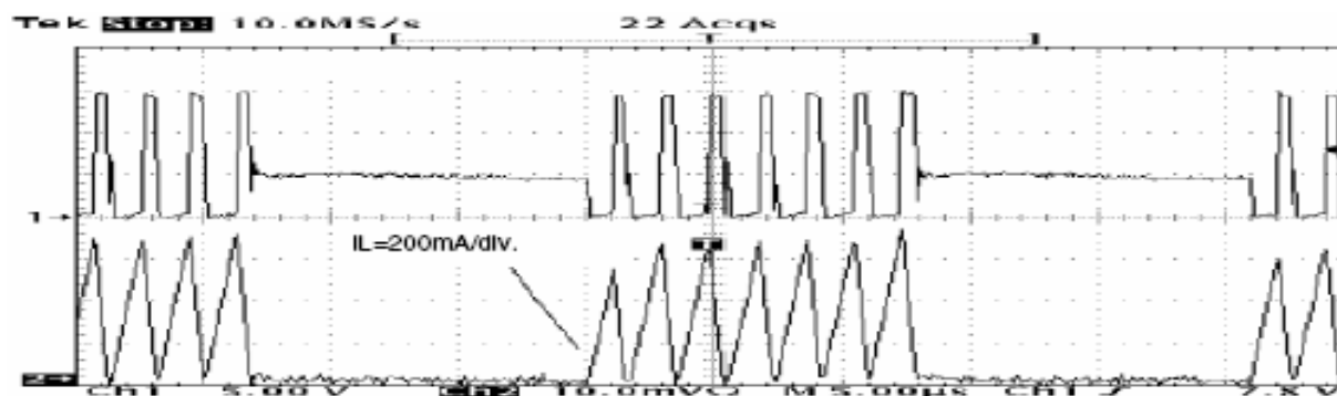
Figure 3: Switching Waveform
