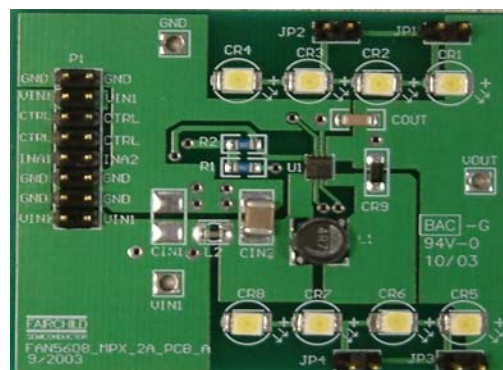
Figure 2: FAN5608 MPX/DMPX
