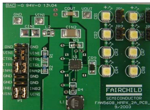
Figure 1: FAN5608 HMPX/DHMPX
