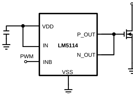
Figure 29. Inverting Application
