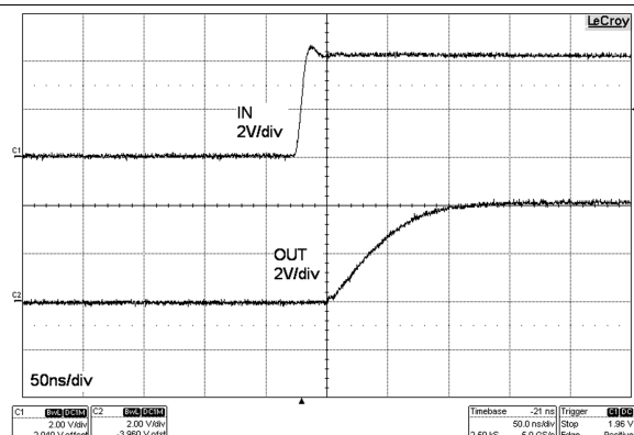
Figure 18. Input Voltage vs Output Voltage ( V_{DD} = 4\text{ V} , C_L = 10000\text{ pF} )
