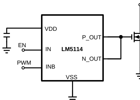
Figure 31. Inverting Application With Enable Pin
