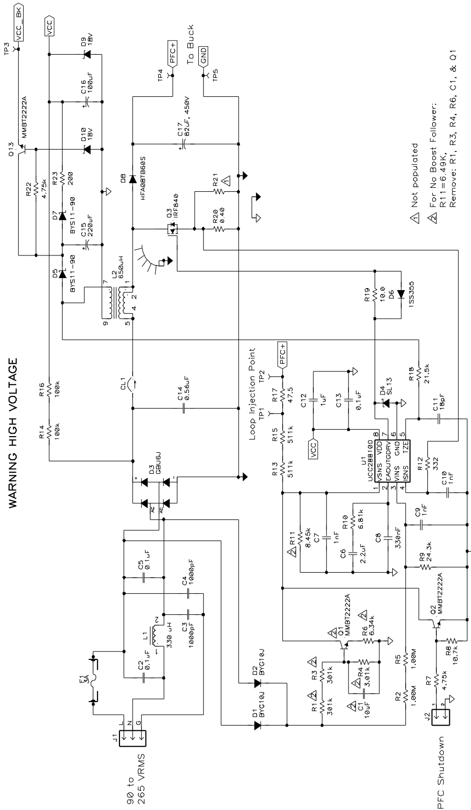
Figure 2. UCC28810EVM-003 PFC Stage Schematic
