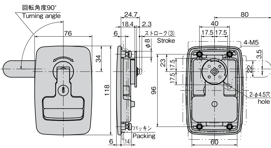
A-244-2-1 (鍵付き) With lock
