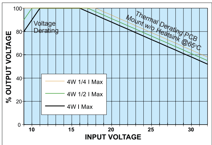
Fig. C Output Voltage vs. 12V/4 Watt Extended Input Voltage (Up to 65°C Chassis Mount w/o Heatsink)
