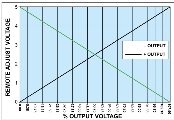
Fig. E Remote Control Characteristics
