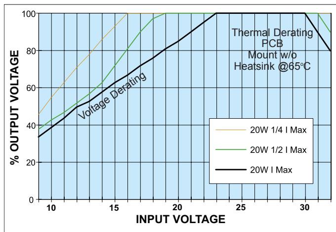
Fig. D Output Voltage vs. 24V/20 Watt Extended Input Voltage (Up to 65°C Chassis Mount w/o Heatsink)
