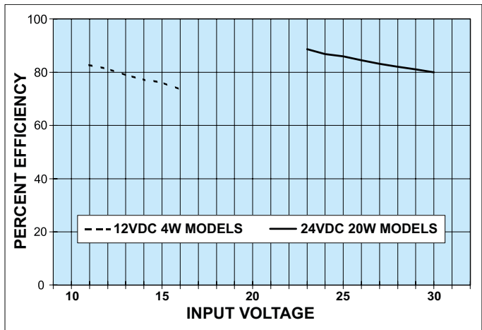
Fig. A DC Efficiency vs. Input Voltage Range
