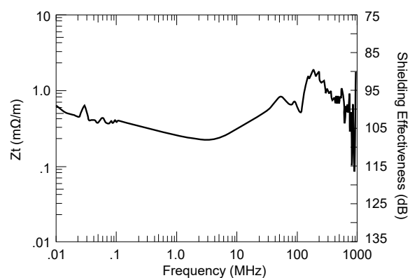
Transfer Impedance
