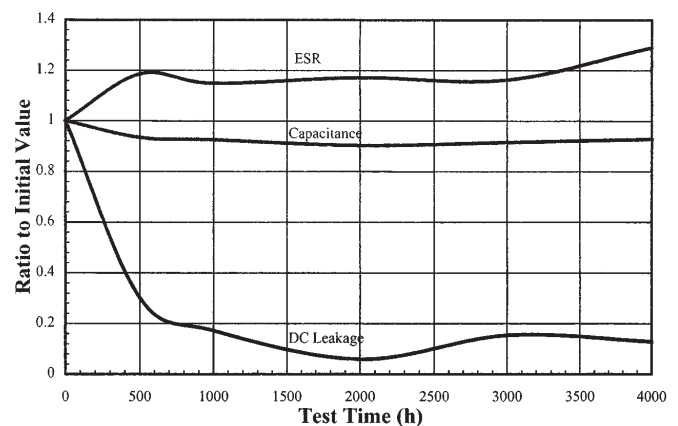
Life Test 15 \mu\text{F} 450 V 105 °C, 556150U450FH2
