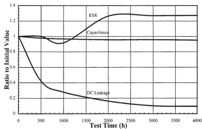
Life Test 22 \mu\text{F} 450 V 105 °C, 556220U450LV2
