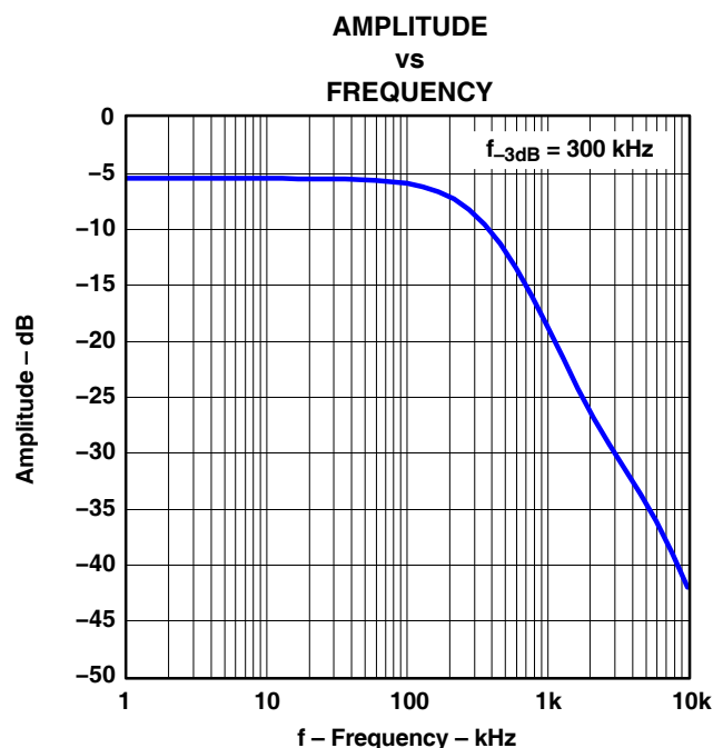
Figure 8. Antialiasing Filter Stop-Band Characteristics
