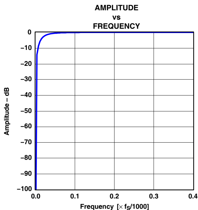
Figure 6. HPF Stop-Band Characteristics
