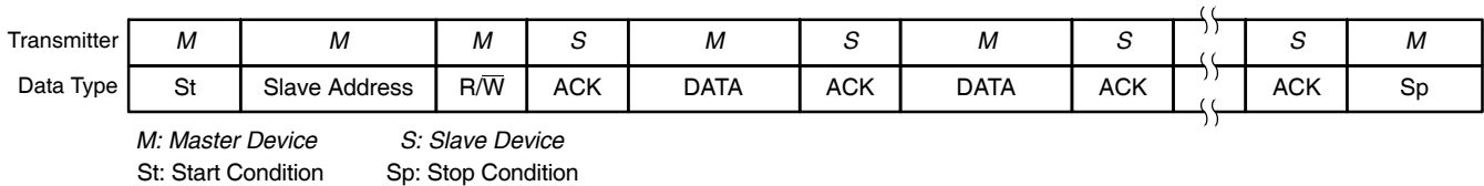
Figure 30. Basic I 2 C Framework
