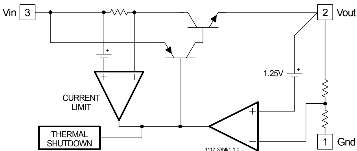
Figure 2 - Simplified block diagram of the IRU1117-33
