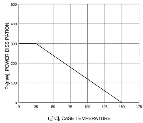
Figure 8. Power Derating
