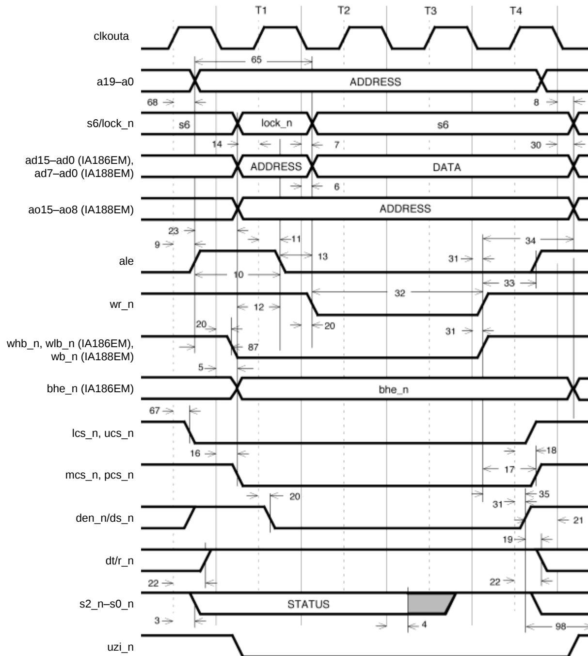
Figure 13. Write Cycle
