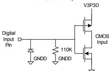
Digital Input
