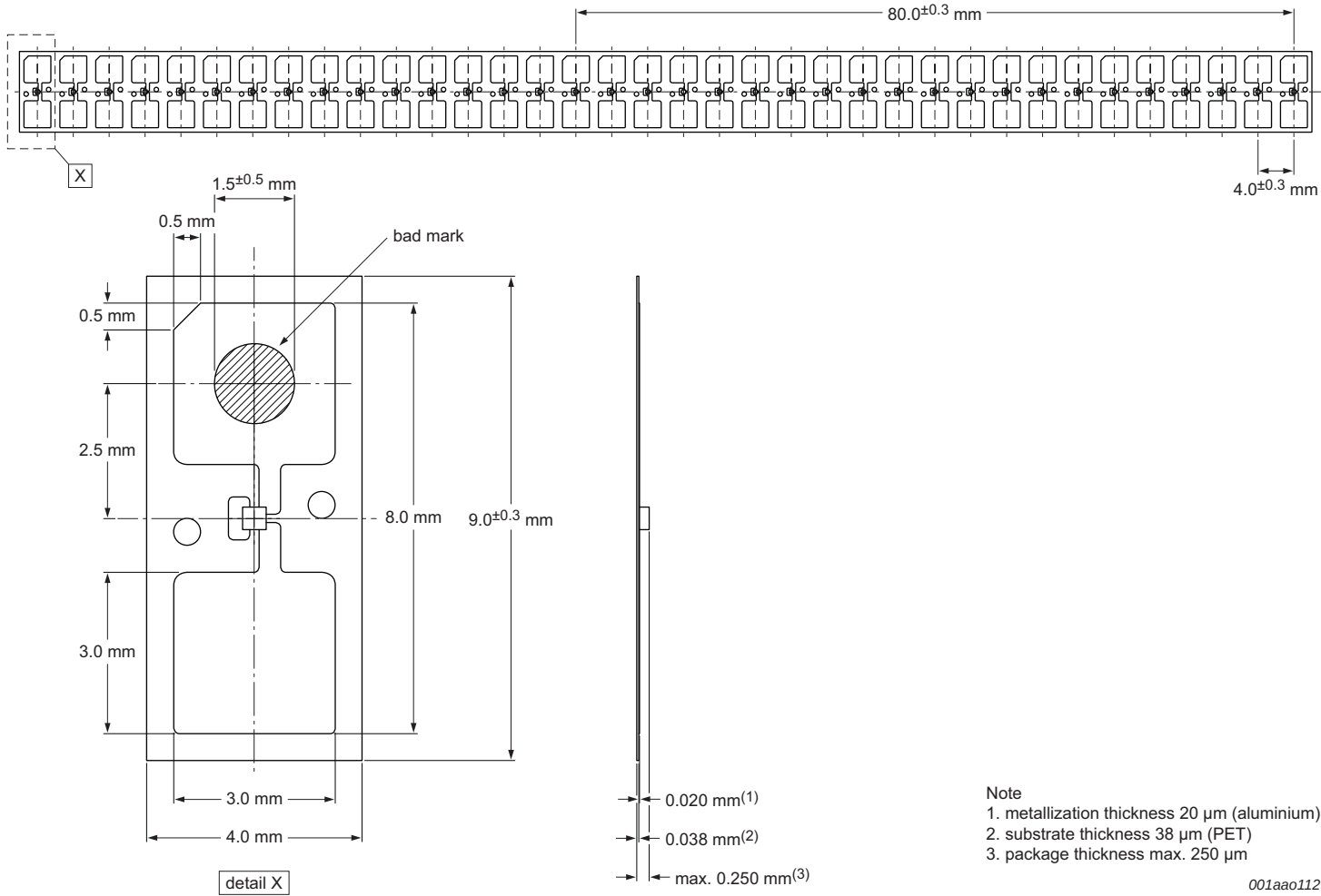
Fig 10. Package FCS2, SOT1040AB2, 20 \mu\text{m} Al metallization
