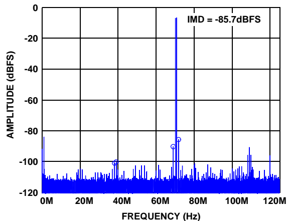
FIGURE 20. TWO-TONE SPECTRUM @ 70MHz
