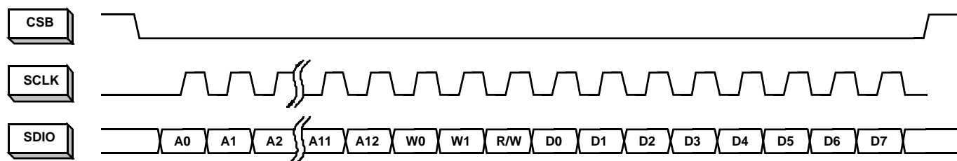
FIGURE 35. LSB-FIRST ADDRESSING
