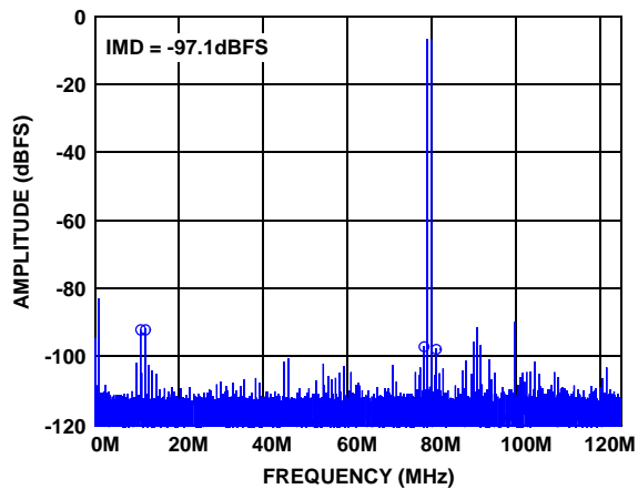
FIGURE 21. TWO-TONE SPECTRUM @ 170MHz
