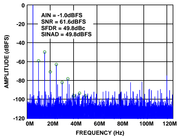
FIGURE 19. SINGLE-TONE SPECTRUM @ 995MHz
