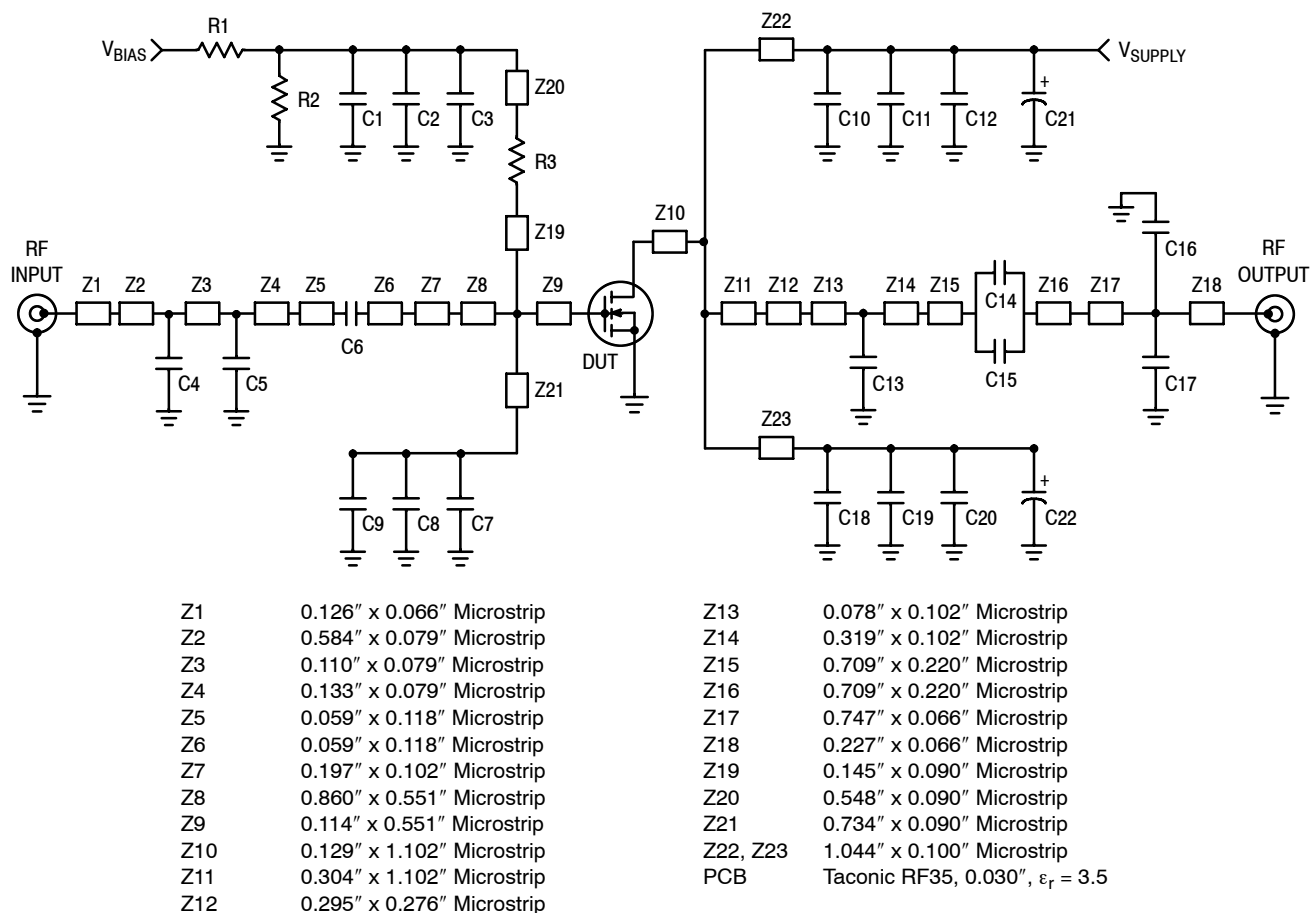
Figure 1. MRF7S19210HR3(HSR3) Test Circuit Schematic
