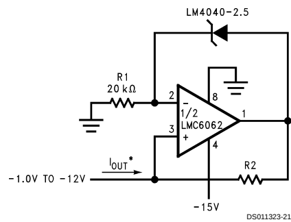
FIGURE 6. Precision 1 μA to 1 mA Current Sources
