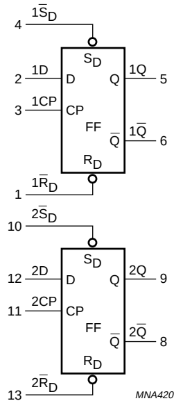
Fig.4 Functional diagram.
