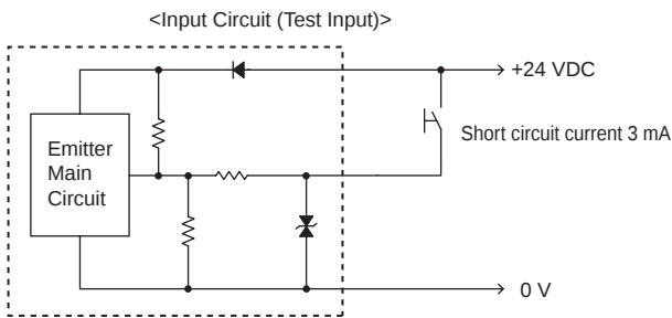
Input circuit diagram by function
