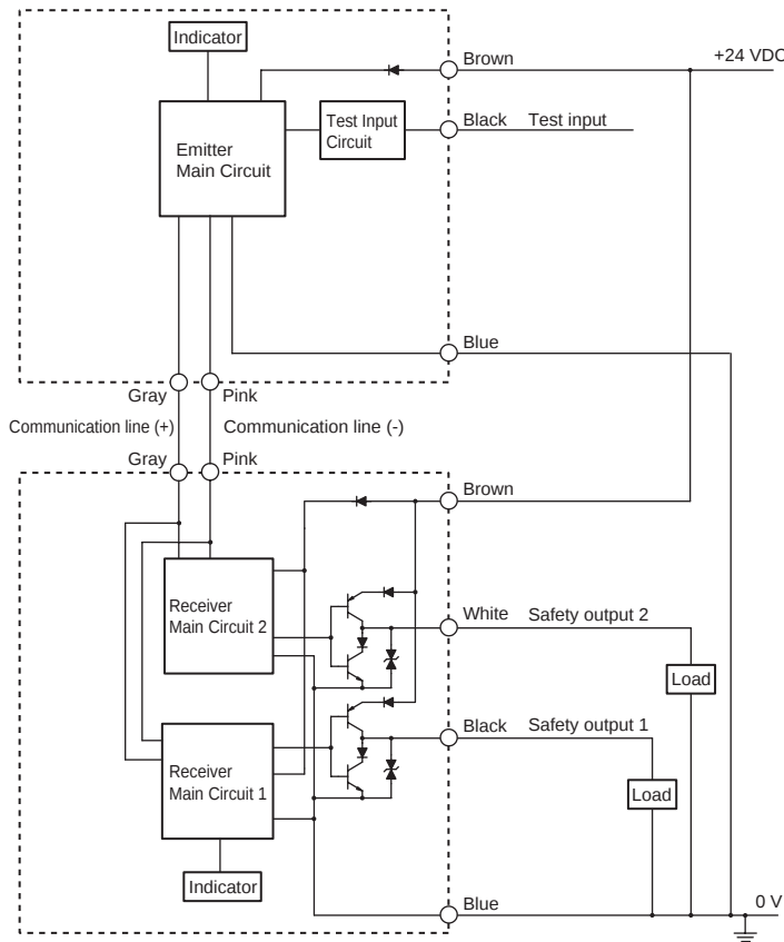
Entire Circuit Diagram
