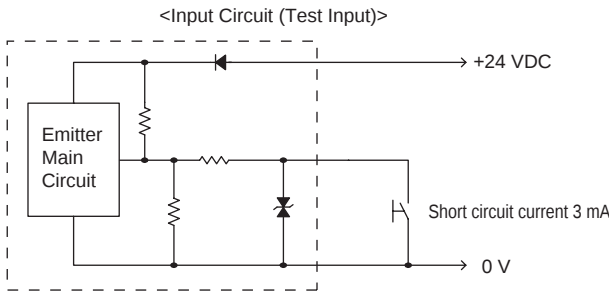
Input circuit diagram by function
