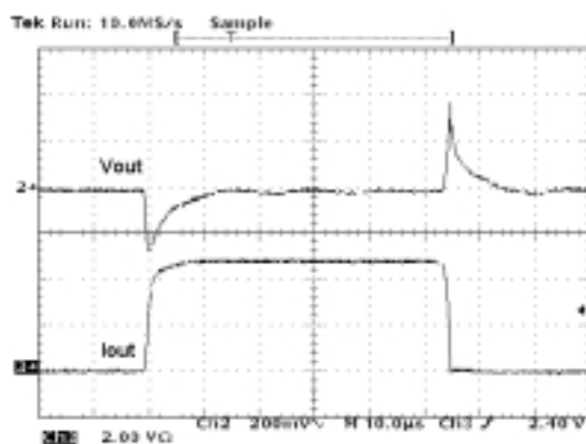
Figure 26: Load Transient
