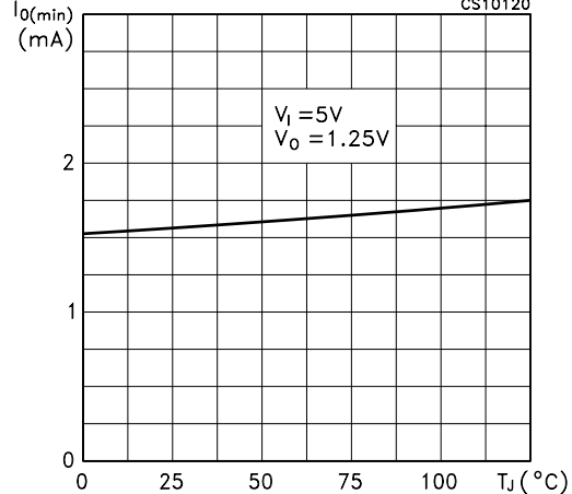
Figure 17: Minimum Load Current vs Temperature
