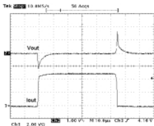
Figure 25: Load Transient
