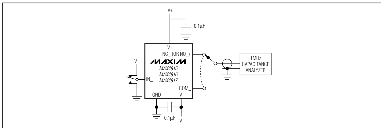
Figure 5. Channel Off-/On-Capacitance
