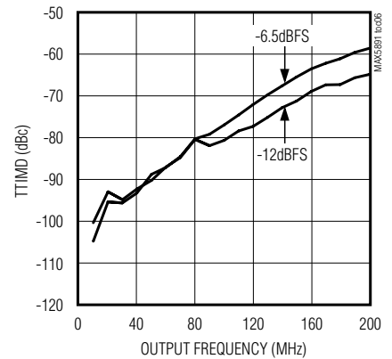
TWO-TONE INTERMODULATION DISTORTION vs. OUTPUT FREQUENCY (f CLK = 500MHz, 1MHz CARRIER SPACING)
