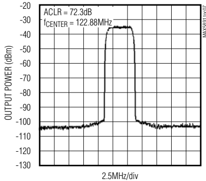
SINGLE-CARRIER WCDMA ACLR (fCLK = 491.52MHz)
