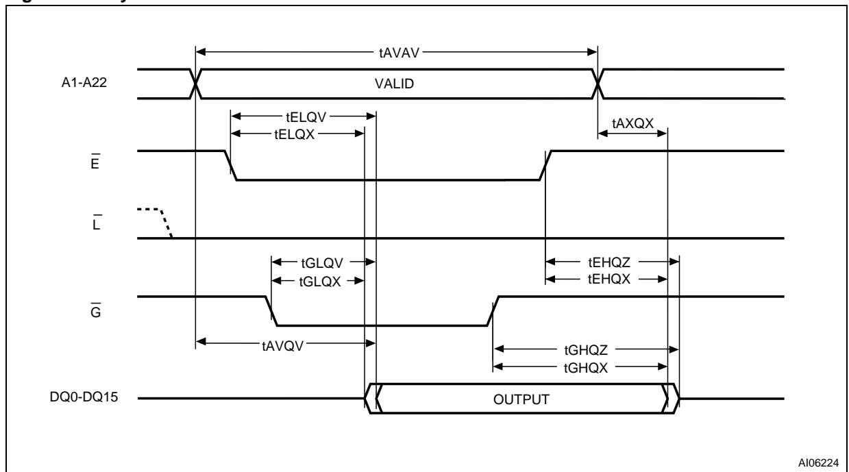
Figure 11. Asynchronous Random Read AC Waveforms
