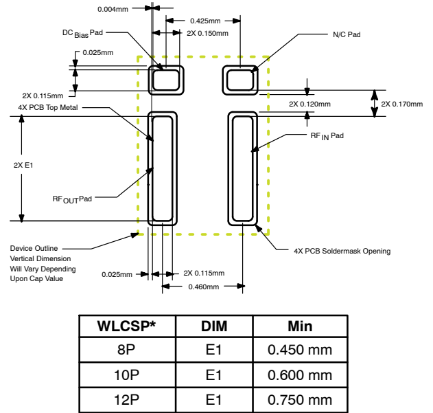
Figure 8. Recommended Pad Layout
