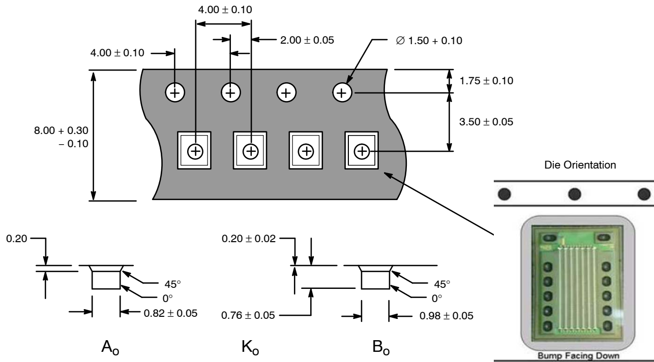
Figure 11. 12 Pillar WLCSP Carrier Tape Drawing
