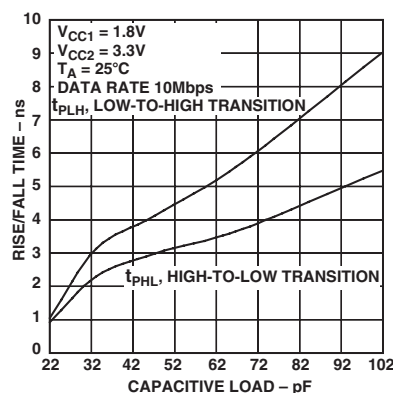
TPC 15. Rise/Fall Time vs. Capacitive Load, A1-Y1, A2-Y2
