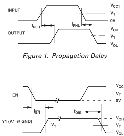
Figure 2. Y1 Enable and Disable Times
