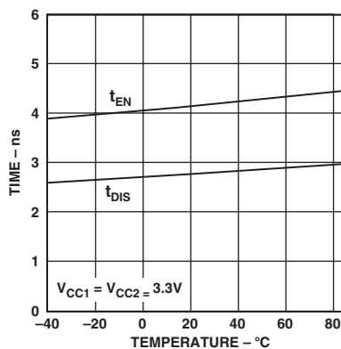
TPC 11. Y1 Enable, Disable Time vs. Temperature
