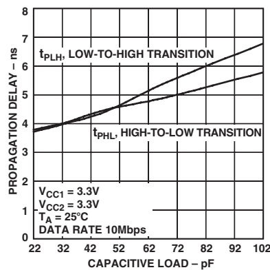
TPC 18. Propagation Delay vs. Capacitive Load A2 to Y2
