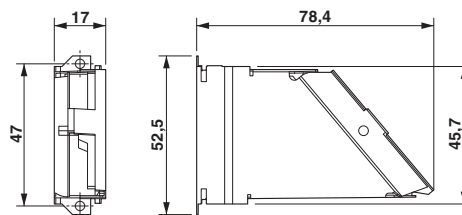
D-SUB EMC inner sleeve
