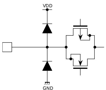
<Analog Switch Input/Output>
