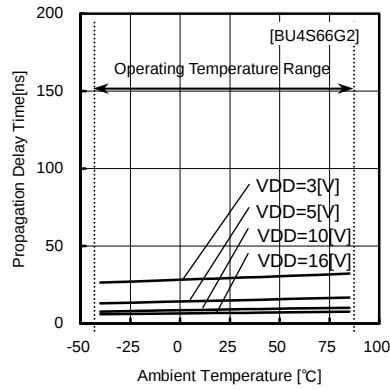
Fig.2 Propagation delay tPLH (IN-OUT)
