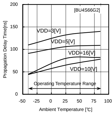
Fig.5 Propagation delay tPLZ (CONT-OUT)
