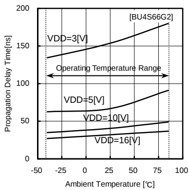
Fig.7 Propagation delay tPZL (CONT-OUT)
