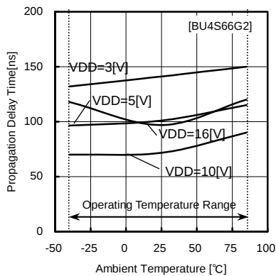
Fig.4 Propagation delay tPHZ (CONT-OUT)
