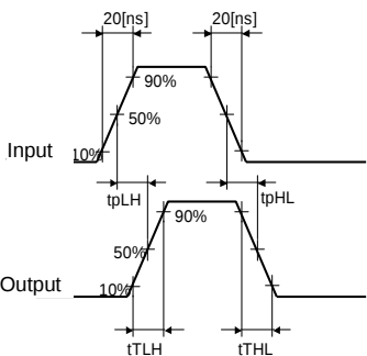
Switching Characteristics
