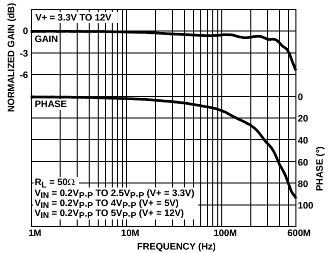
FIGURE 16. FREQUENCY RESPONSE
