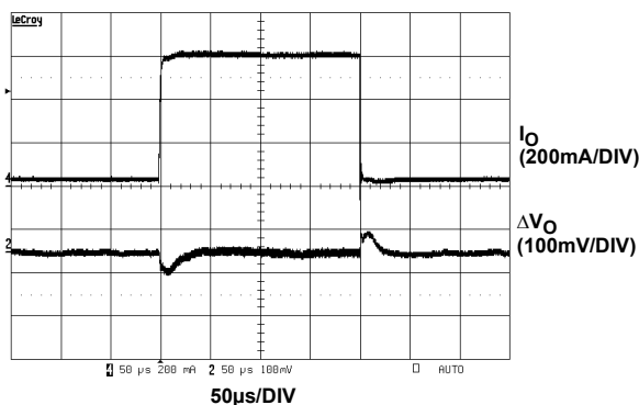
FIGURE 10. LOAD TRANSIENT RESPONSE (30mA TO 600mA)
