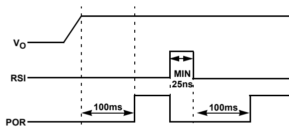
FIGURE 13. RSI AND POR TIMING DIAGRAM
