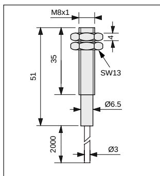
M8 screened
