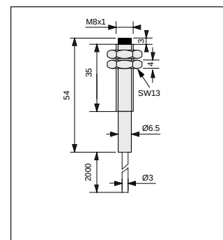
M8 non-screened
