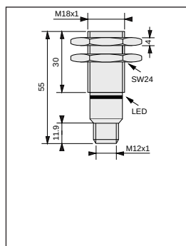
M18 screened
