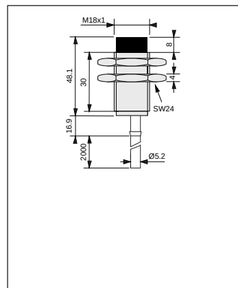
M18 non-screened
