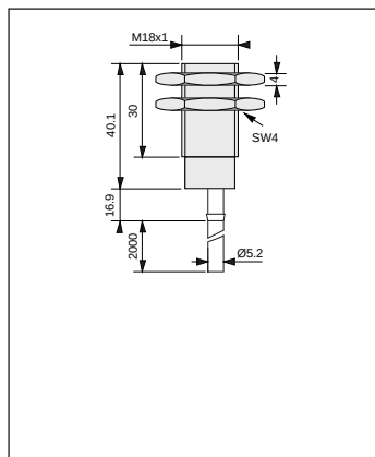
M18 screened
