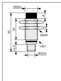
M18 non-screened
